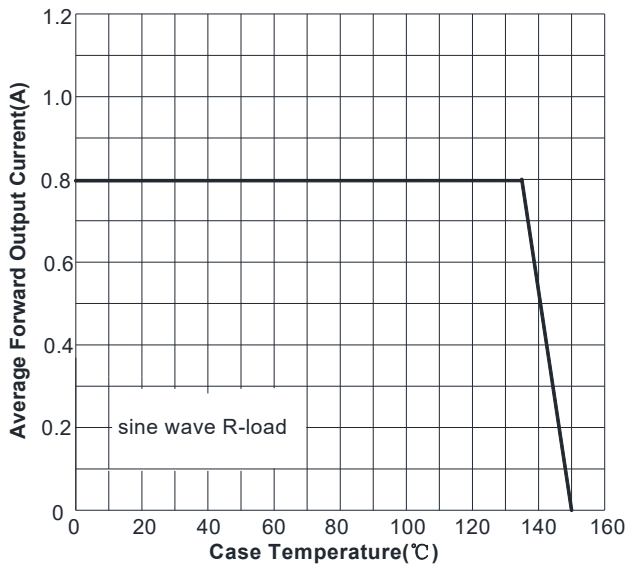
FIG1:Io-Tc Curve
